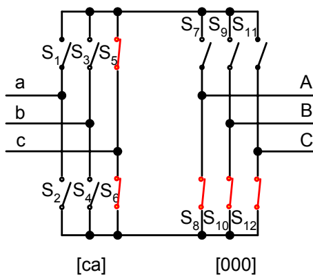
Fig. 1.19 V_0 - I_0 pair during d_0
