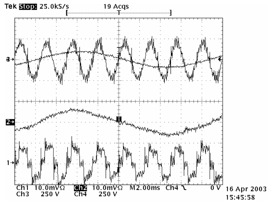
Fig. 4.13 Input/out waveforms at 400Hz (ch1: I_A (20A/div), ch2: I_a (20A/div), ch3: V_A , ch4: V_a )
