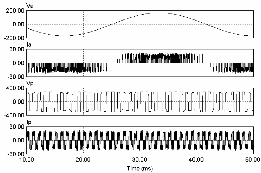
Fig. 4.6 Primary side 3 \phi /1 \phi matrix converter waveforms ( f_{in} = 30 Hz)
