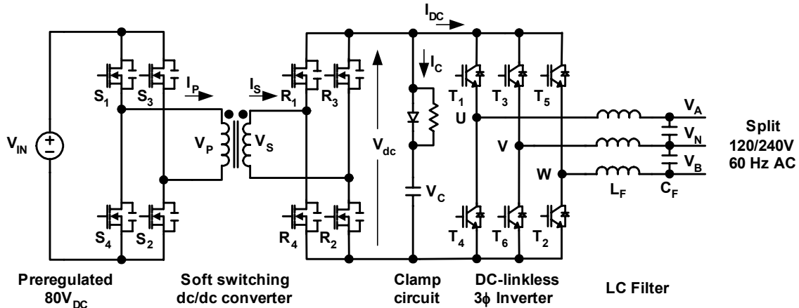
Fig. 5.2 The proposed 1φ/3φ direct converter for resident power system
