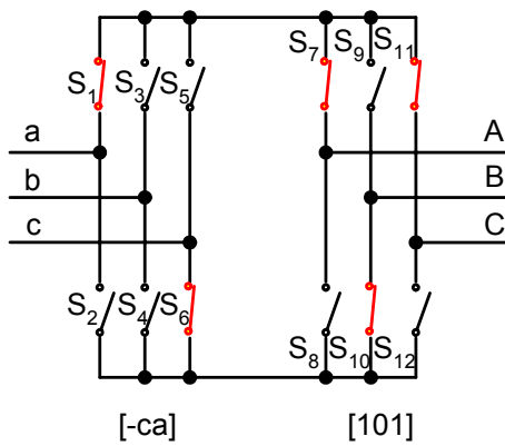
Fig. 1.17 V_6 - I_2 pair during d_{\alpha\delta}
