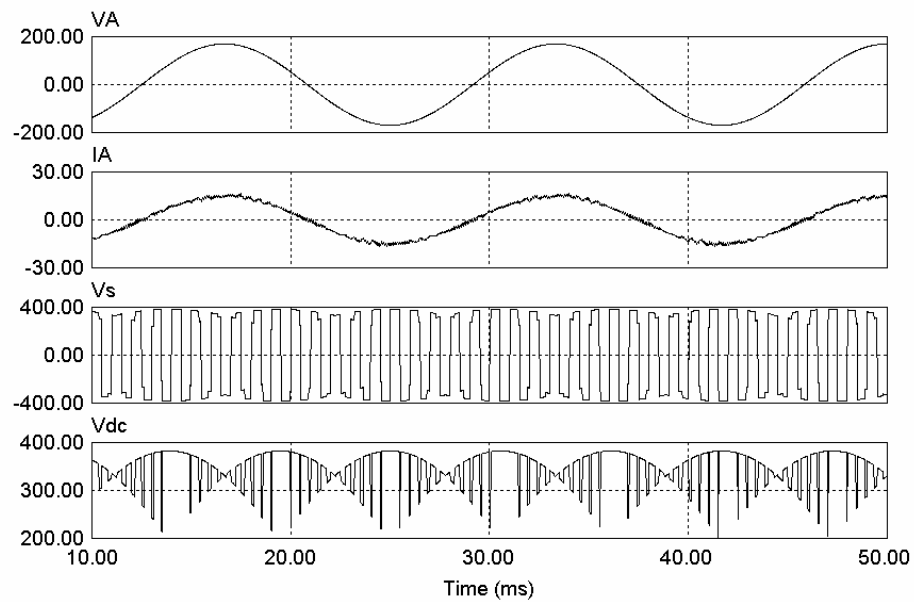
Fig. 4.7 Secondary side 1 \phi /3 \phi matrix converter waveforms ( f_{out} = 60 Hz)
