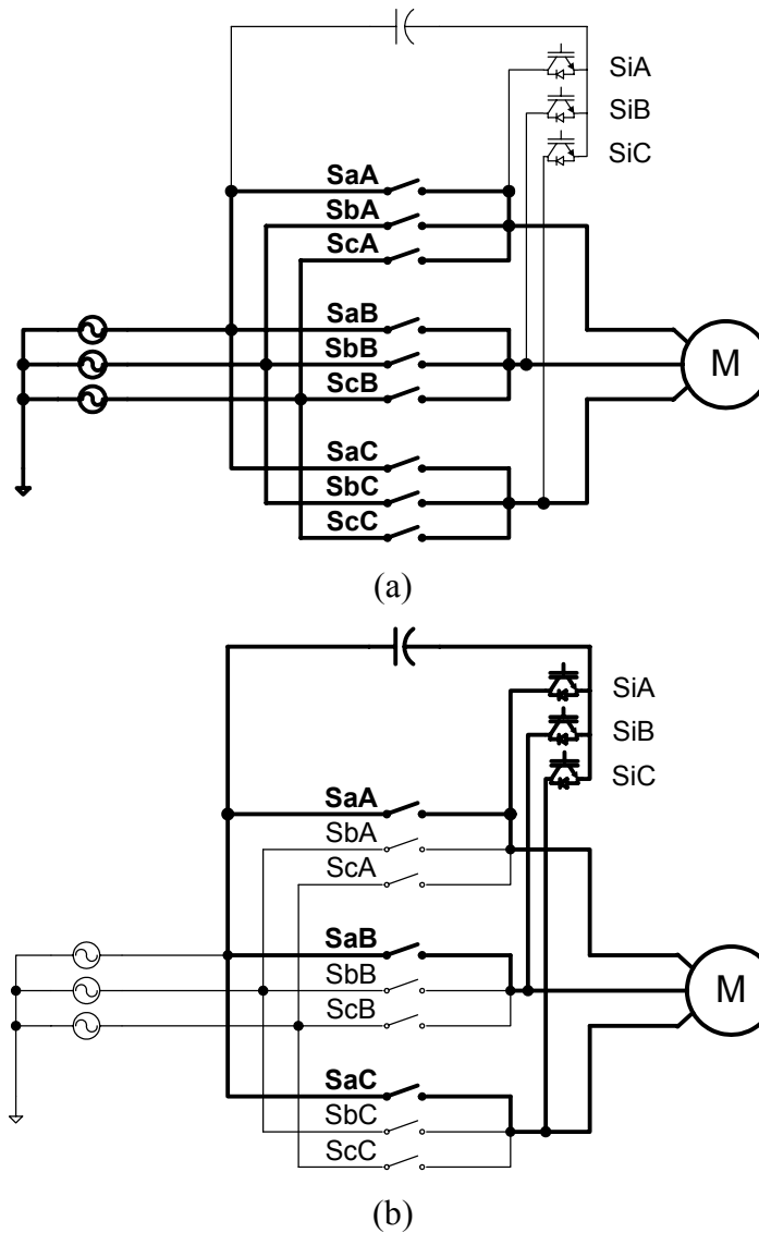
Fig. 3.2 Operating mode (a) normal mode (b) ride-through mode
