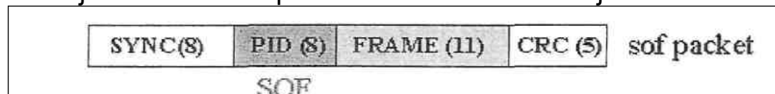
Sl. 13 Format SOF paketa
